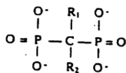
Bisphosphonate
